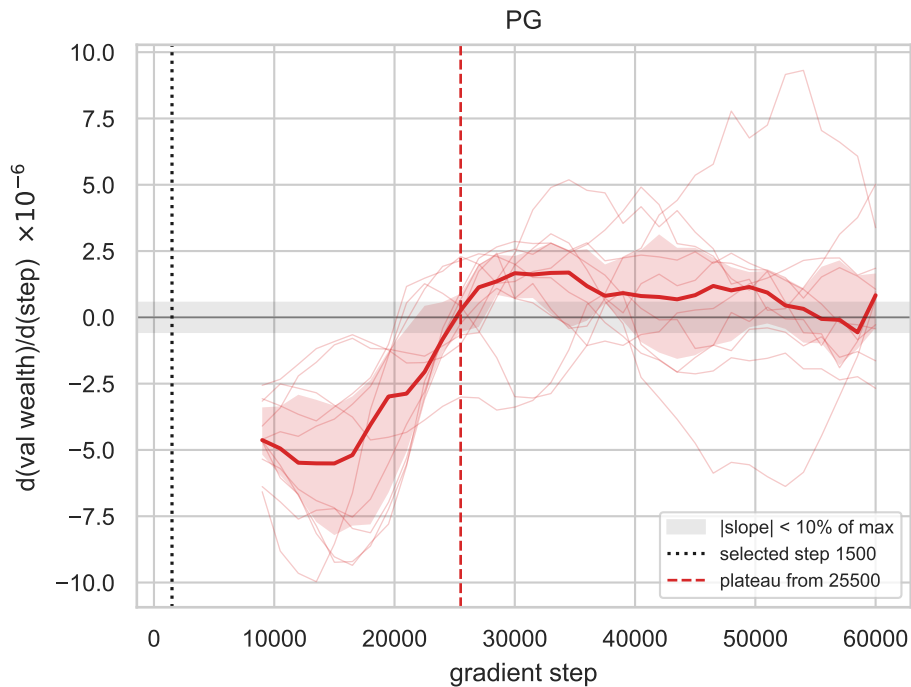
F4 Plateau diagnostic on the validation curve
