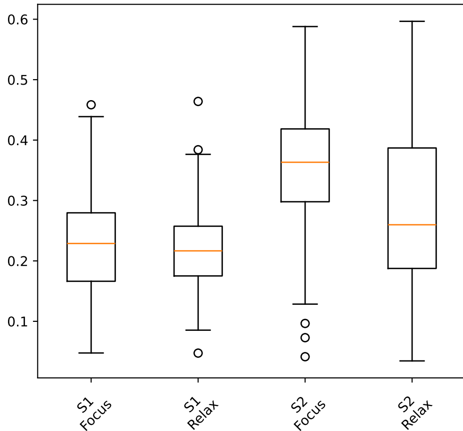
Relative \beta power (W=4s)
