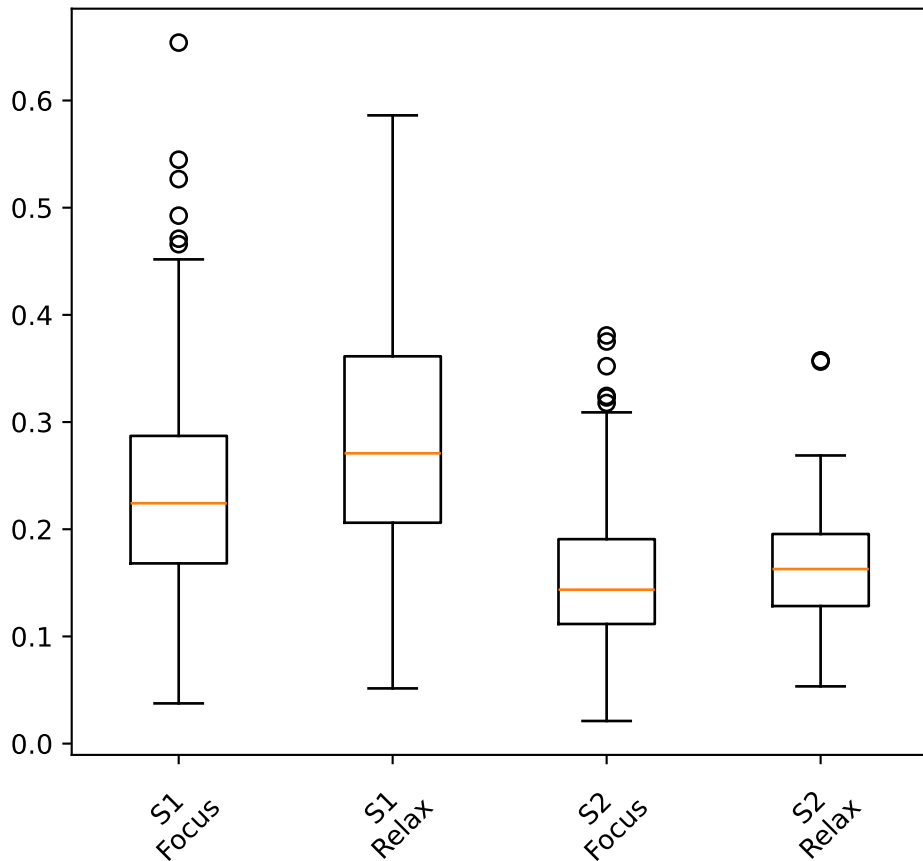
Relative \alpha power (W=4s)
