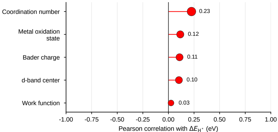
Mechanism feature correlations with \Delta E_{\text{H}^*} (eV)
