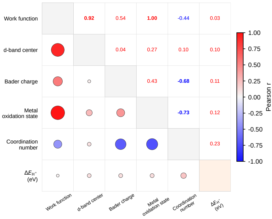
Mechanism correlation matrix for \Delta E_{H^*} (eV)
