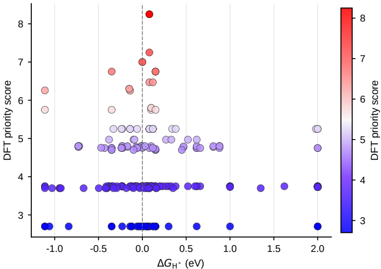
DFT priority score versus \Delta G_{\text{H}^*} (eV)
