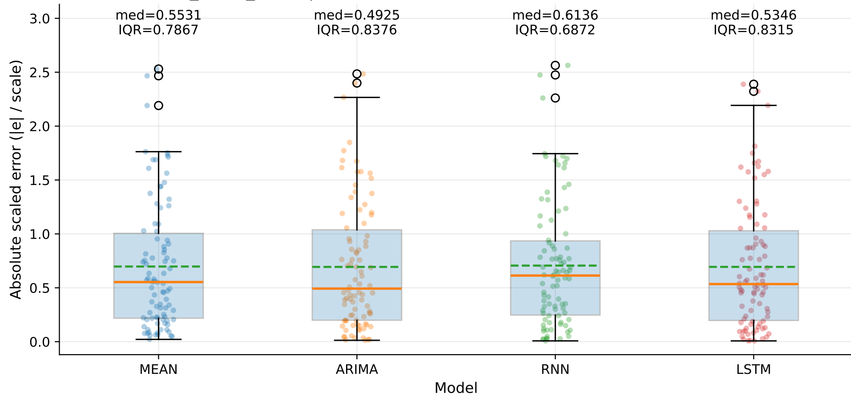
M10_YHUR_SHUR | MASE-point distribution by model — TSEC (step=1)
