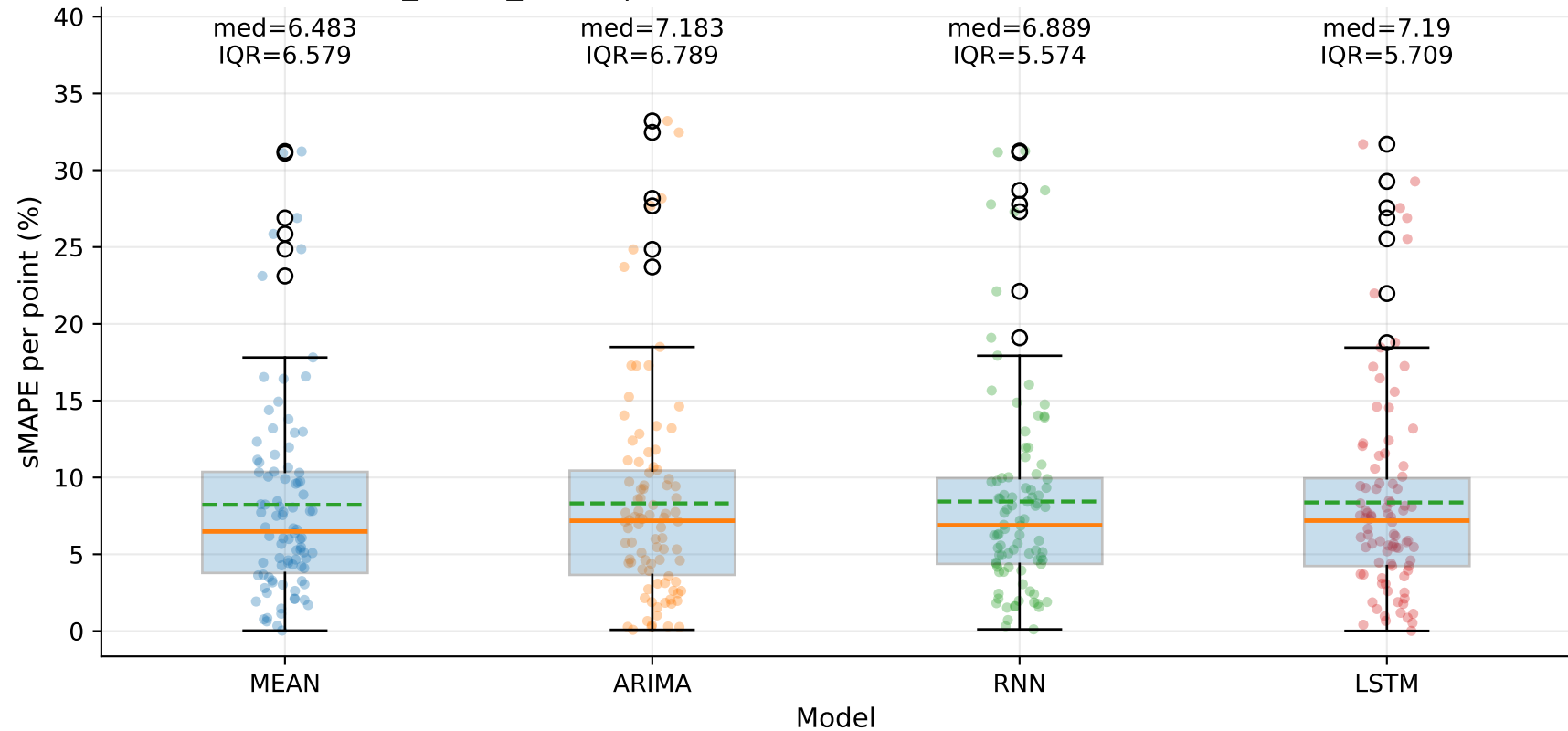
M10_YHUR_SHUR | sMAPE distribution by model — Yd (step=1)
