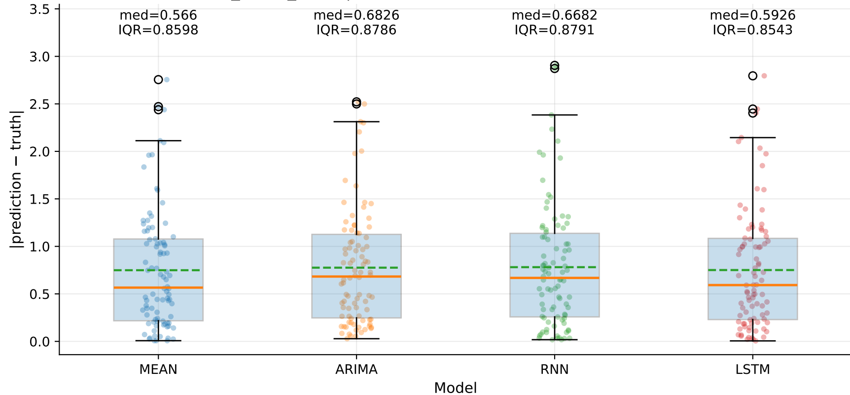
M10_YHUR_SLUR | Absolute error by model — TSEC (step=1)
