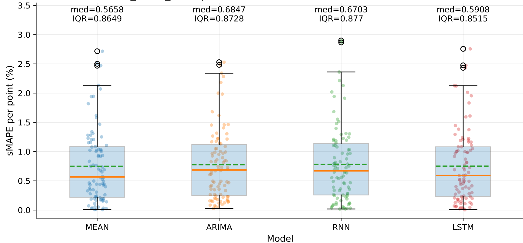
M10_YHUR_SLUR | sMAPE distribution by model — TSEC (step=1)
