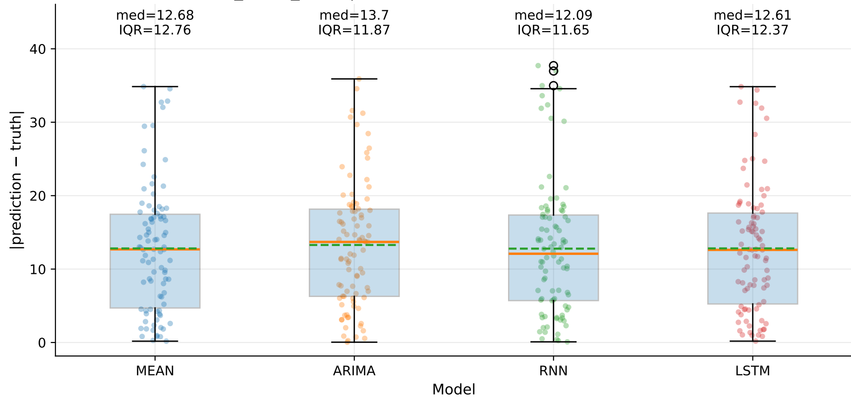
M10_YHUR_SLUR | Absolute error by model — TSE (step=1)
