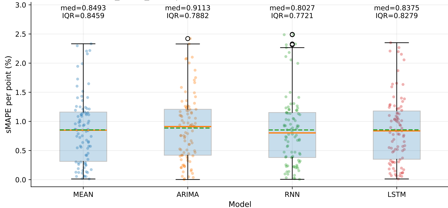
M10_YHUR_SLUR | sMAPE distribution by model — TSE (step=1)
