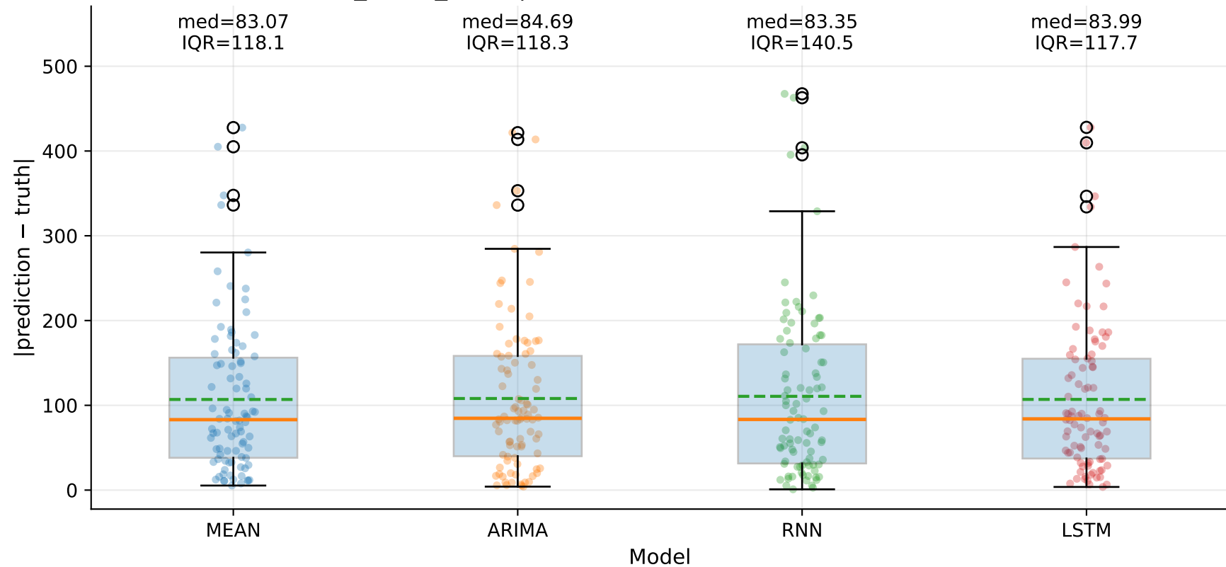
M10_YHUR_SLUR | Absolute error by model — Yd (step=1)
