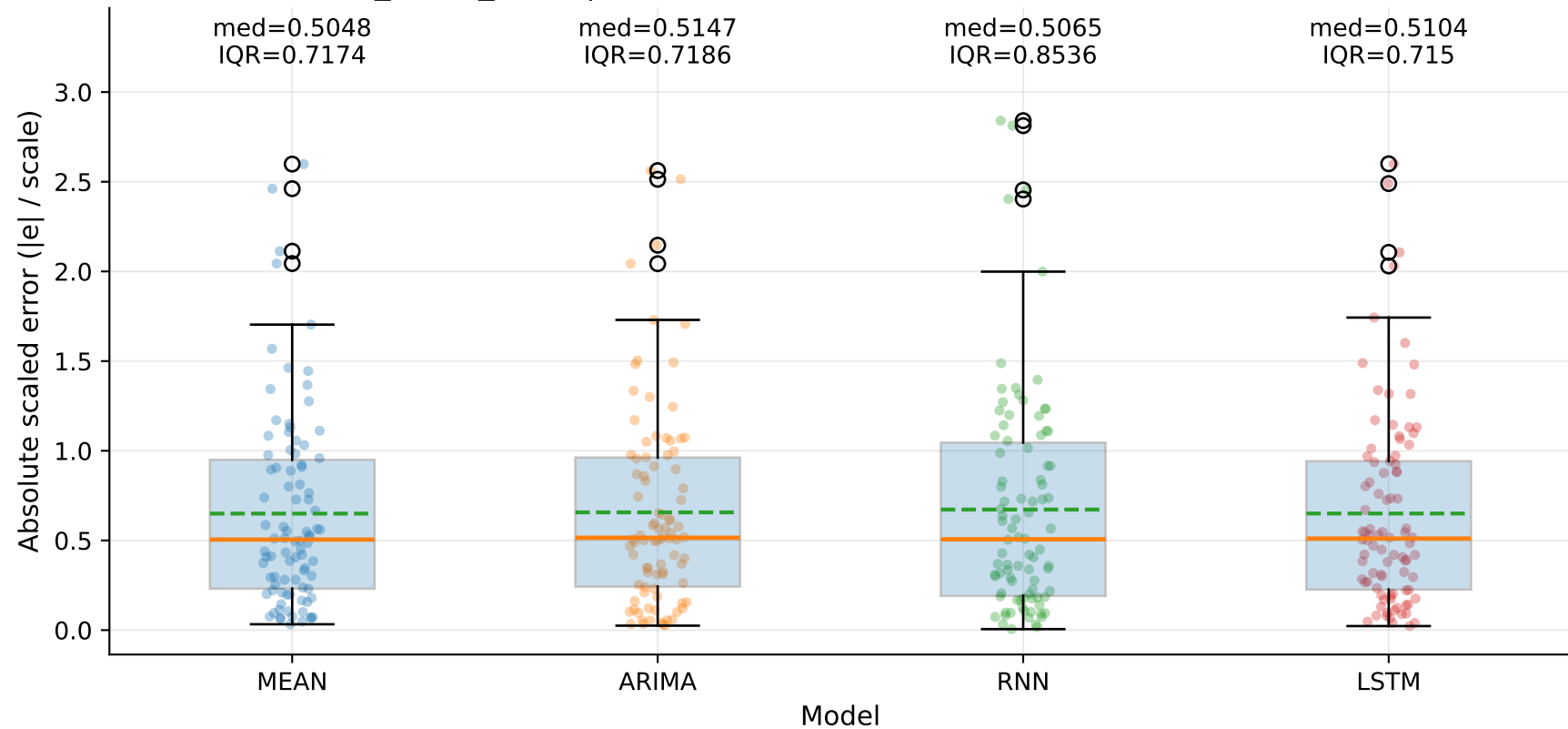
M10_YHUR_SLUR | MASE-point distribution by model — Yd (step=1)
