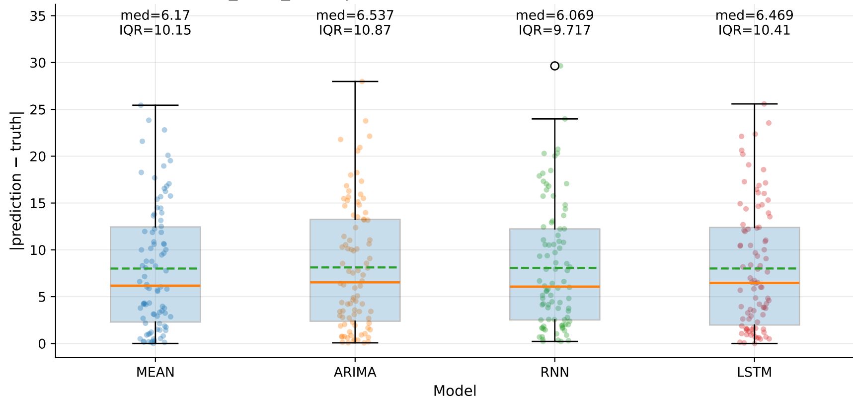
M10_YLUR_SHUR | Absolute error by model — TSEC (step=1)
