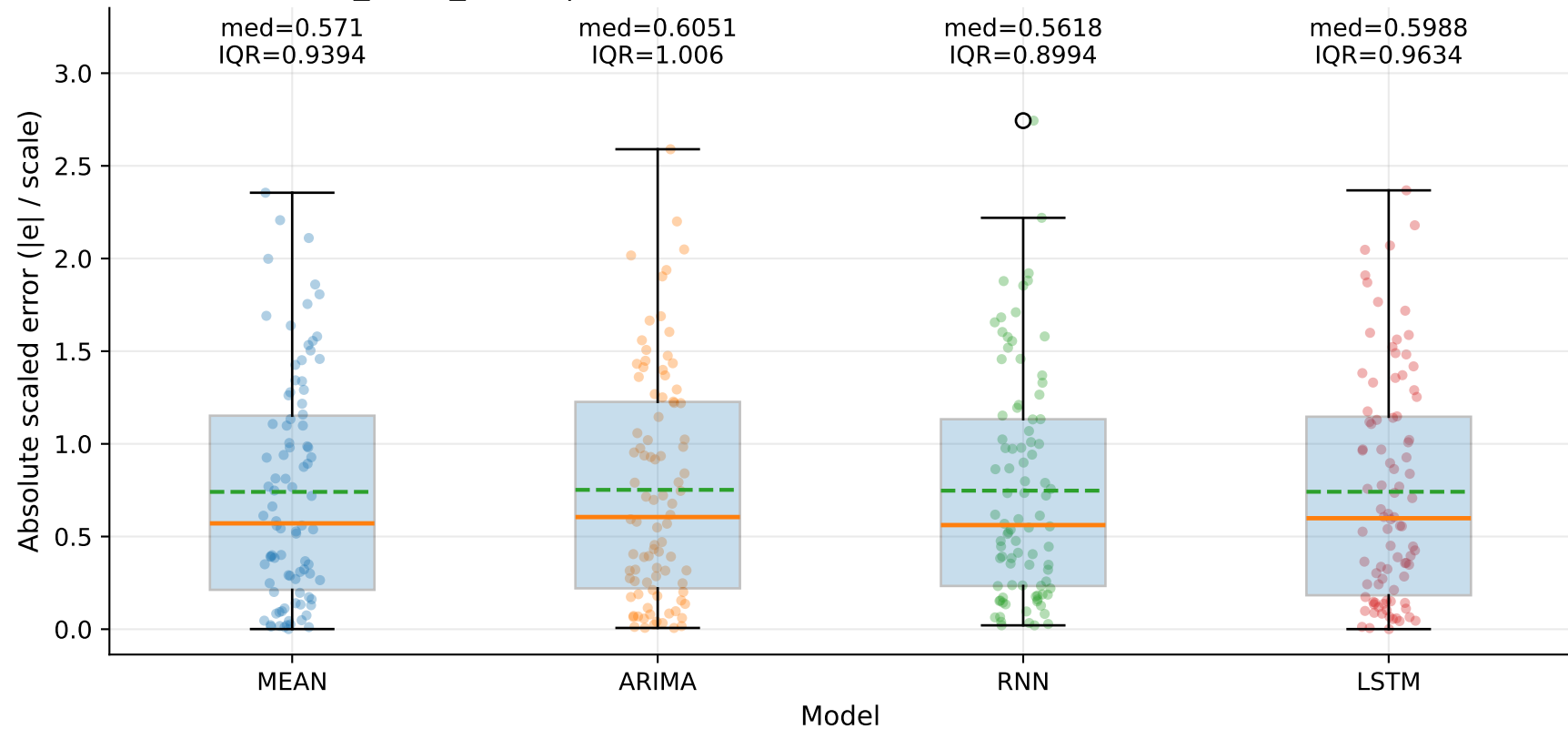
M10_YLUR_SHUR | MASE-point distribution by model — TSEC (step=1)
