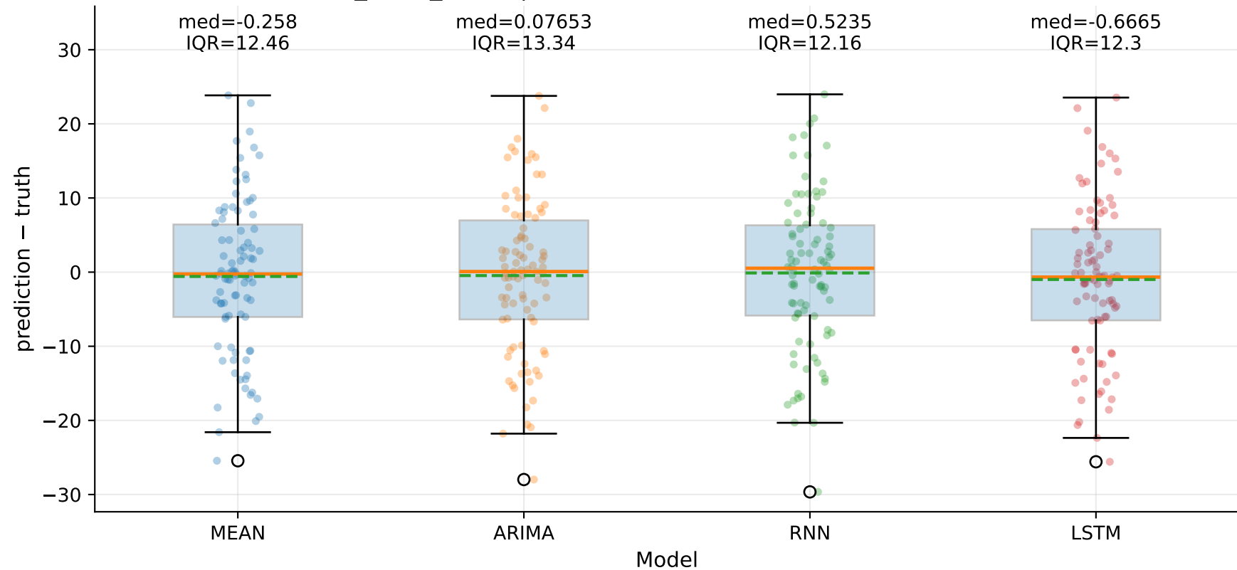
M10_YLUR_SHUR | Signed error by model — TSEC (step=1)
