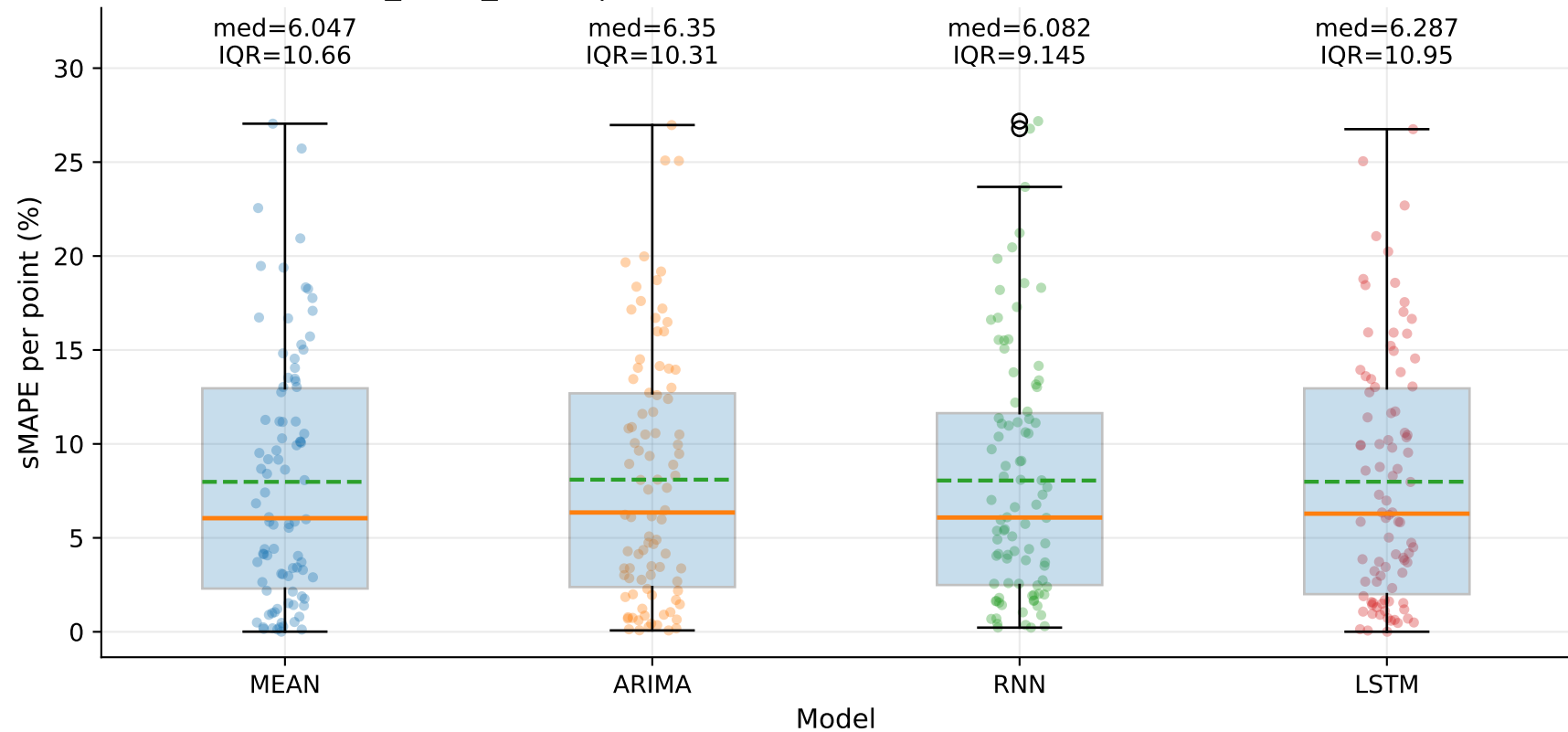
M10_YLUR_SHUR | sMAPE distribution by model — TSEC (step=1)
