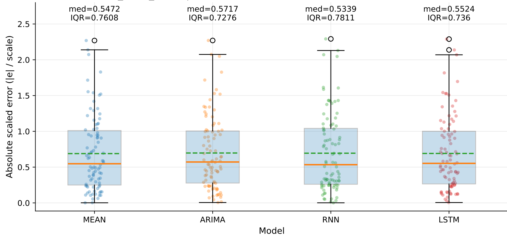
M10_YLUR_SHUR | MASE-point distribution by model — TSE (step=1)
