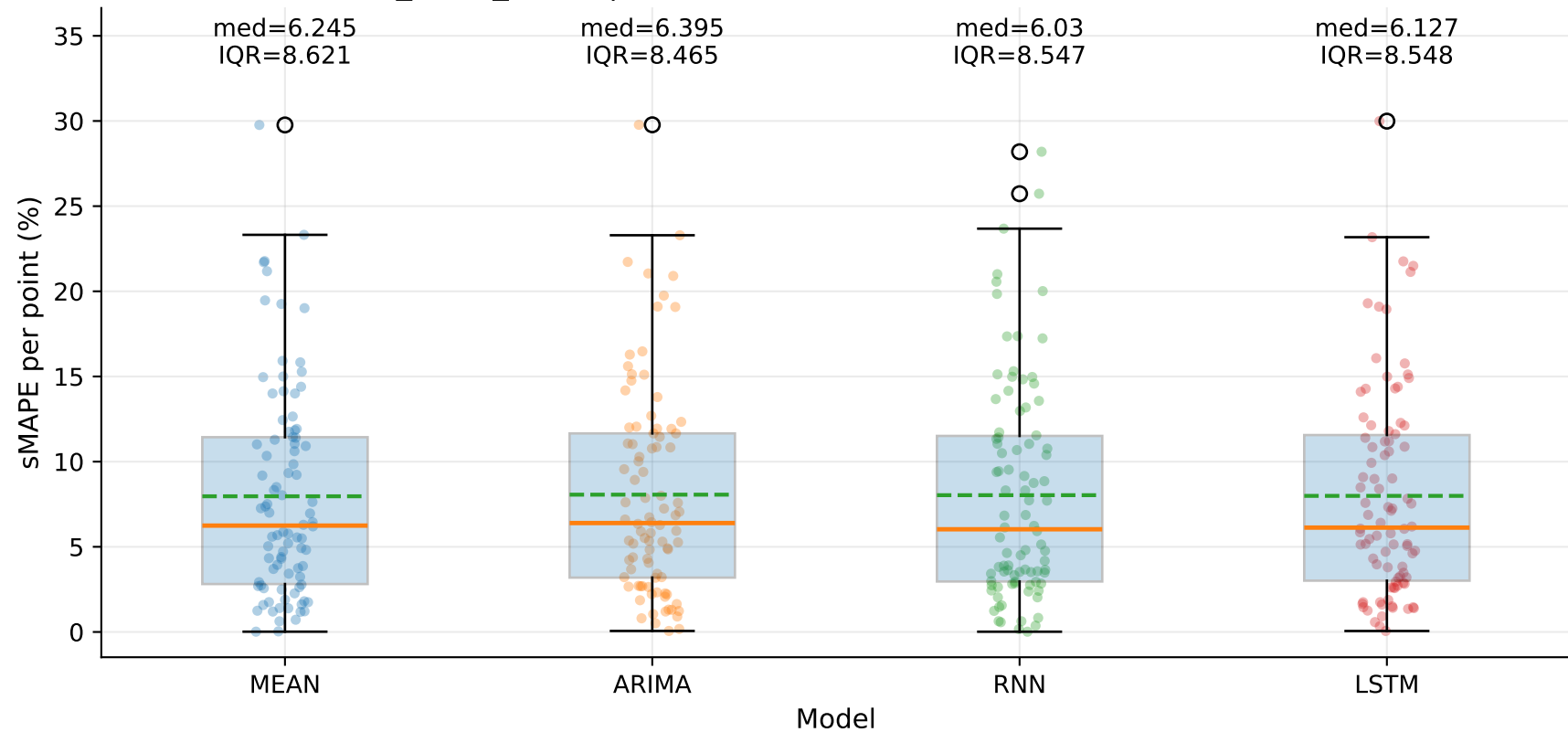
M10_YLUR_SHUR | sMAPE distribution by model — TSE (step=1)
