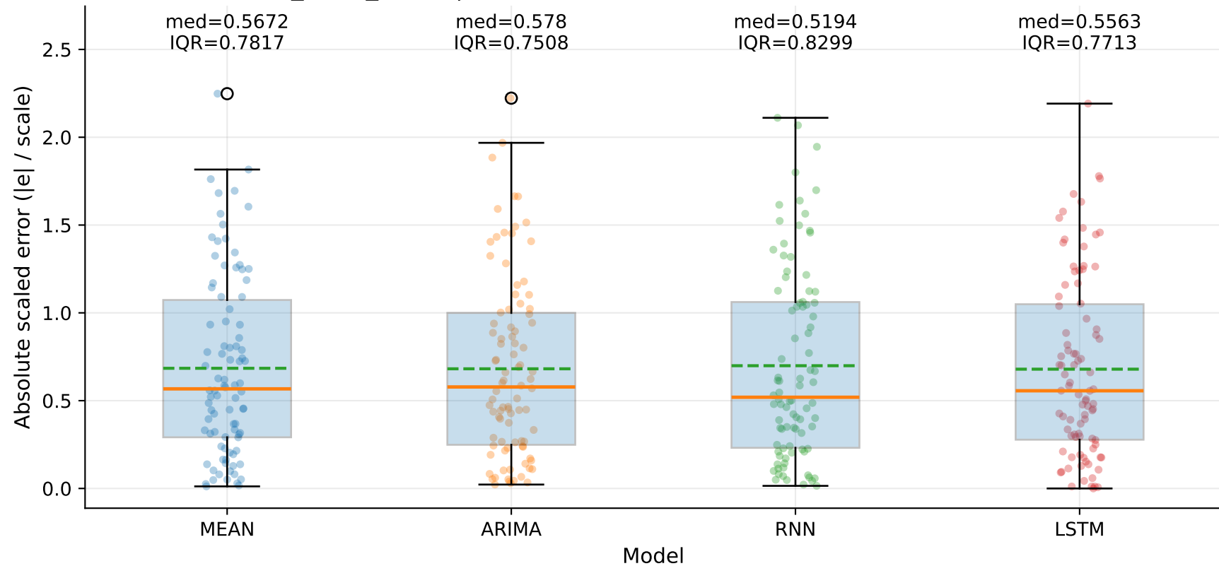
M10_YLUR_SHUR | MASE-point distribution by model — Yd (step=1)
