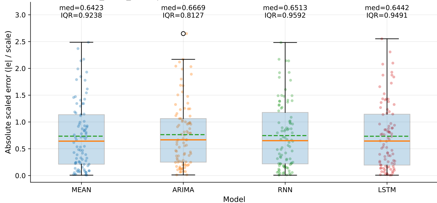
M10_YLUR_SLUR | MASE-point distribution by model — TSEC (step=1)
