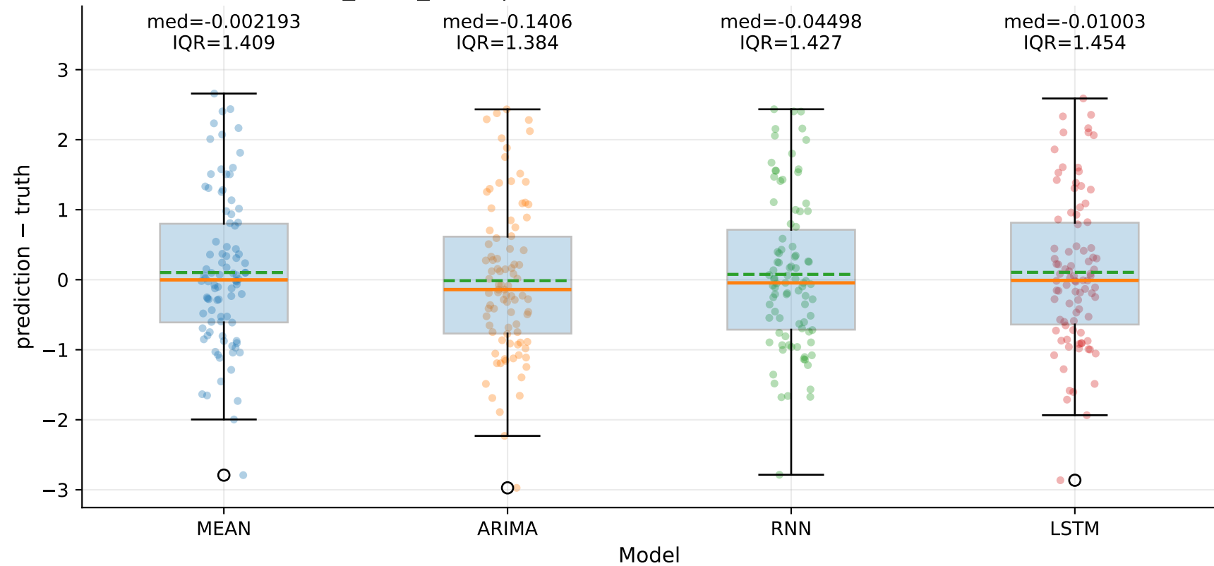
M10_YLUR_SLUR | Signed error by model — TSEC (step=1)
