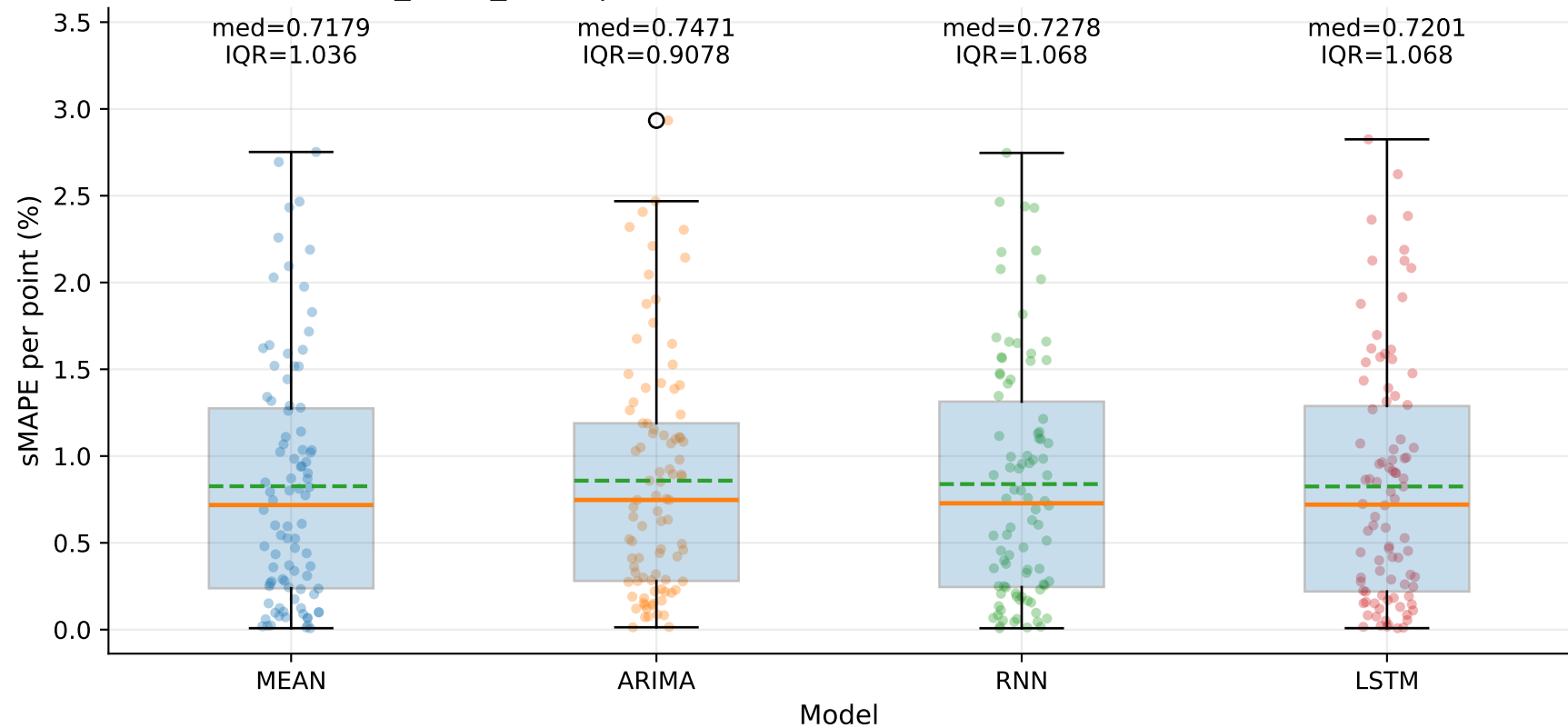
M10_YLUR_SLUR | sMAPE distribution by model — TSEC (step=1)
