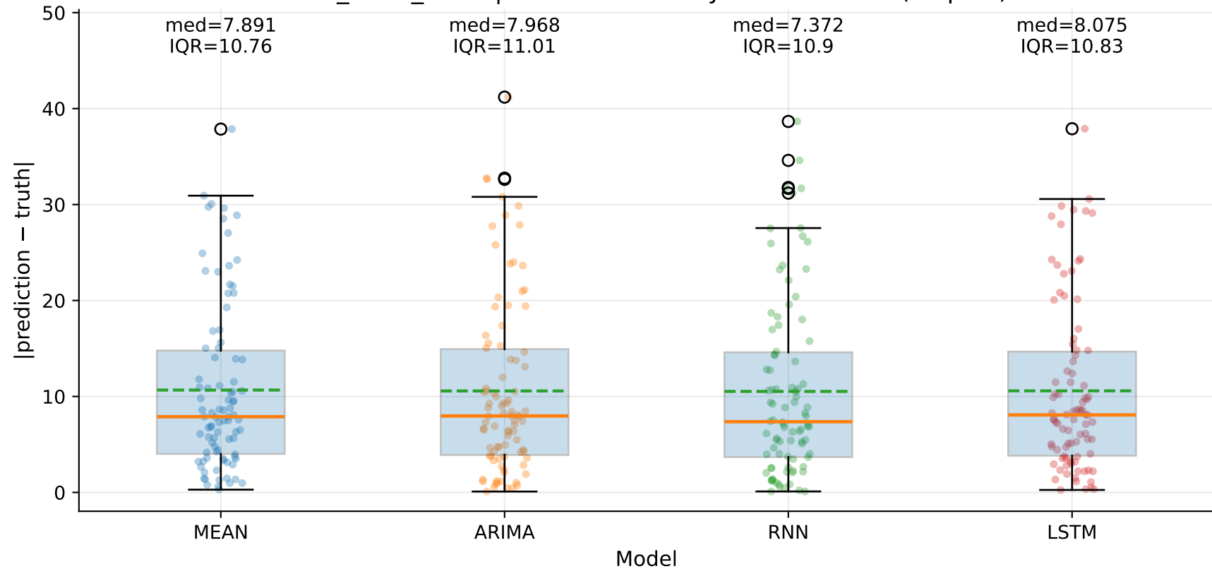
M10_YLUR_SLUR | Absolute error by model — TSE (step=1)
