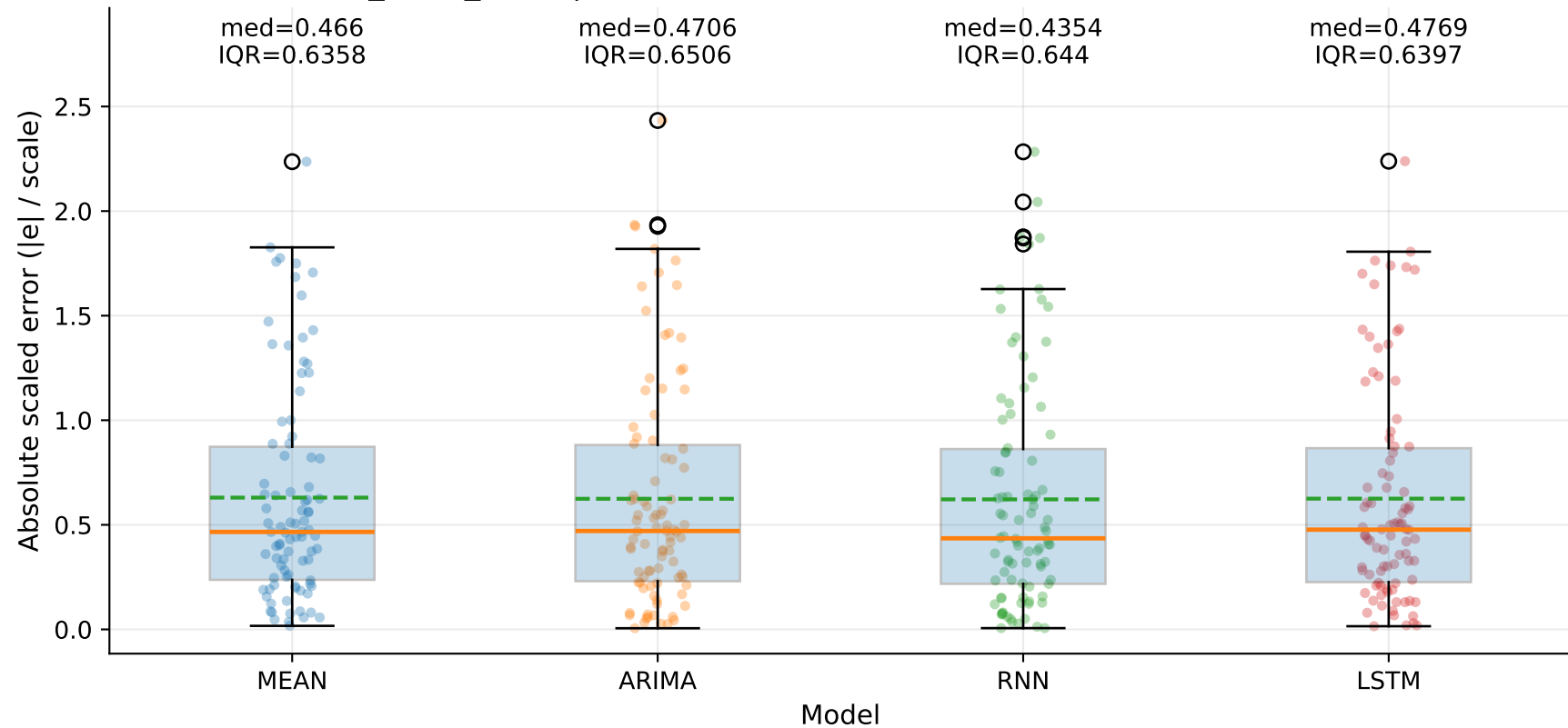
M10_YLUR_SLUR | MASE-point distribution by model — TSE (step=1)
