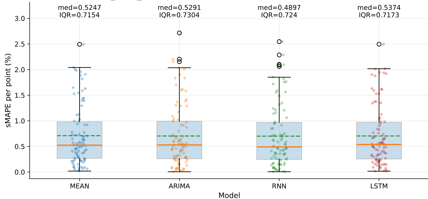
M10_YLUR_SLUR | sMAPE distribution by model — TSE (step=1)
