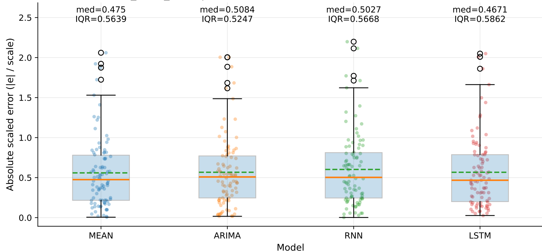
M10_YLUR_SLUR | MASE-point distribution by model — Yd (step=1)
