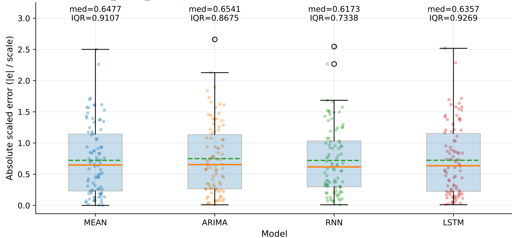
M4_YHUR_SHUR | MASE-point distribution by model — TSEC (step=1)
