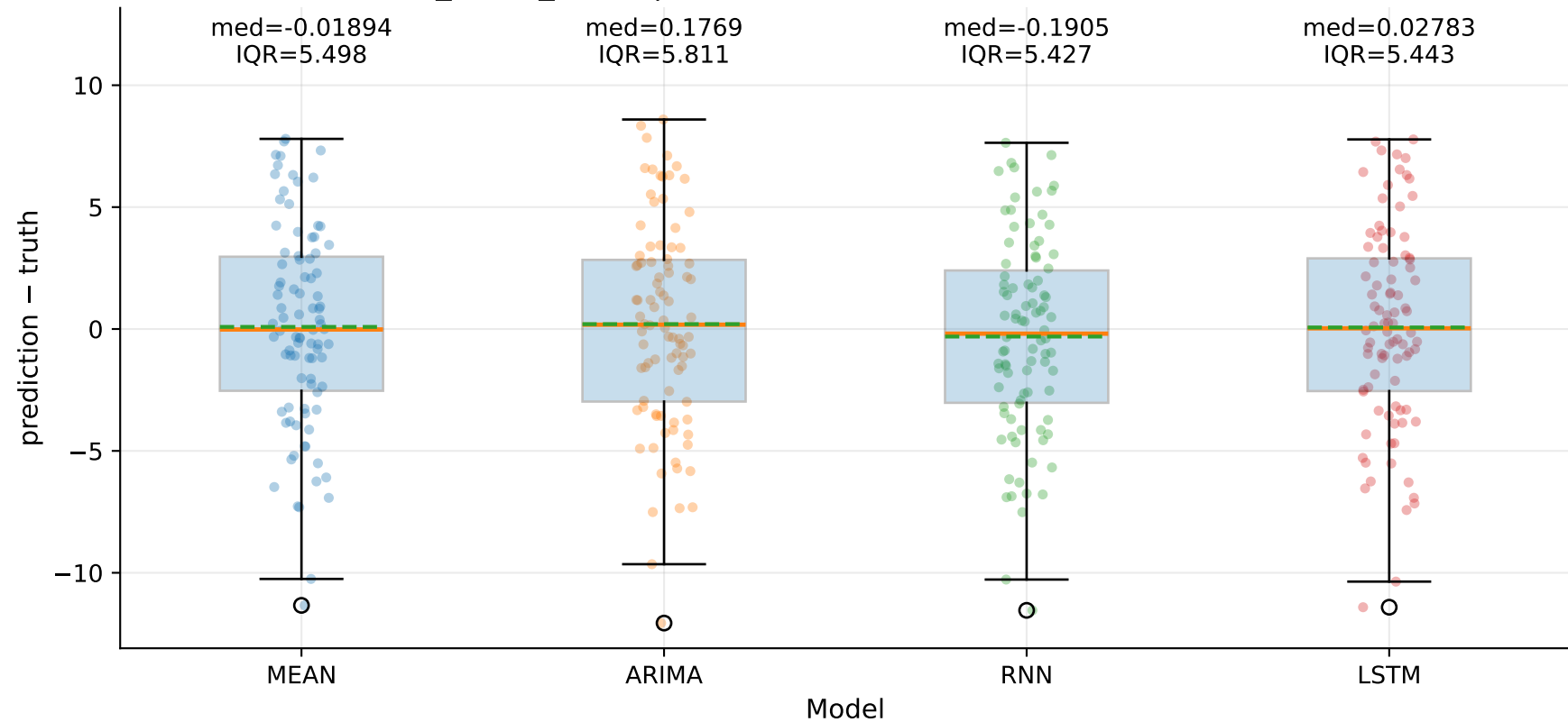
M4_YHUR_SHUR | Signed error by model — TSEC (step=1)
