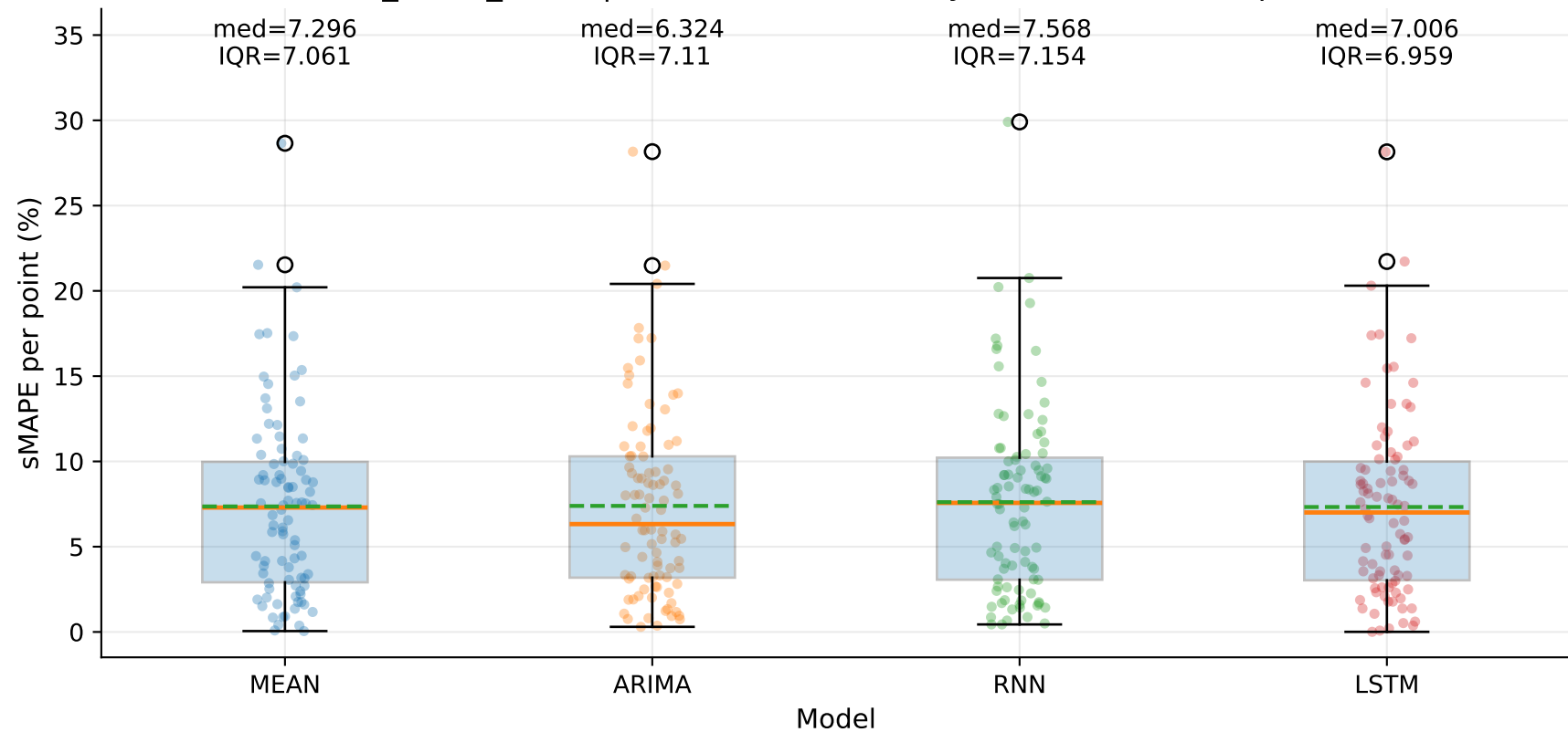
M4_YHUR_SHUR | sMAPE distribution by model — TSE (step=1)
