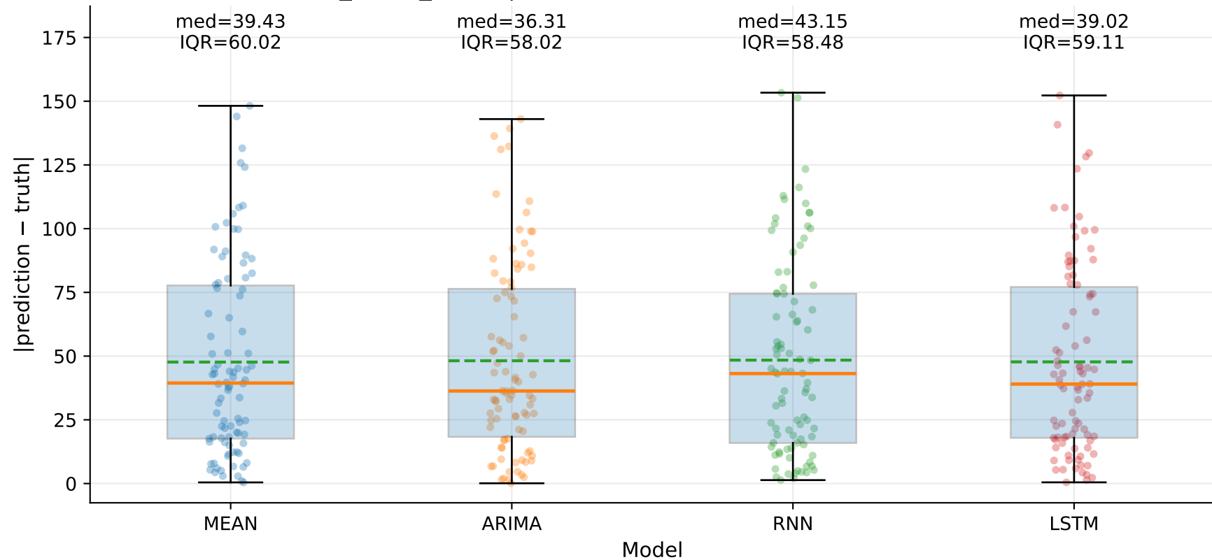
M4_YHUR_SHUR | Absolute error by model — Yd (step=1)
