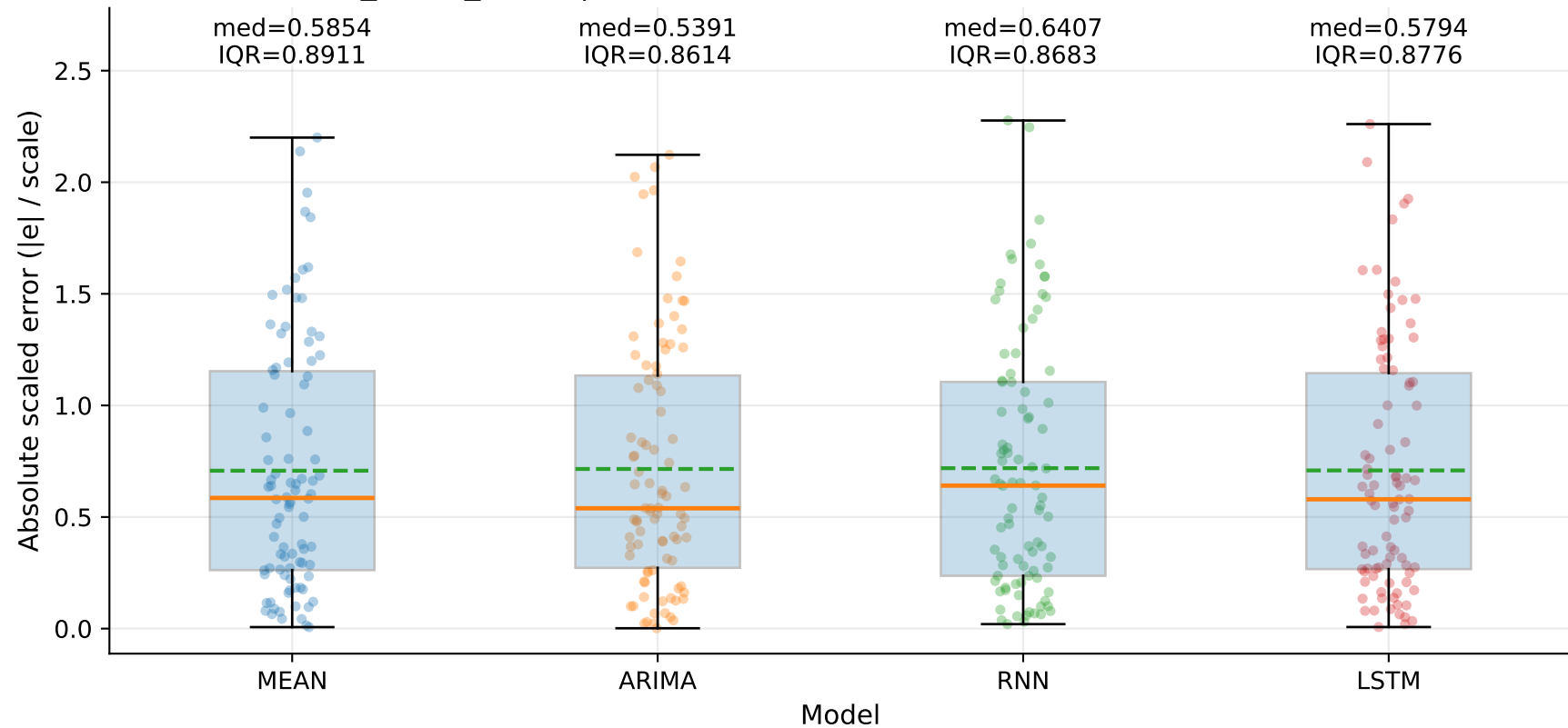
M4_YHUR_SHUR | MASE-point distribution by model — Yd (step=1)
