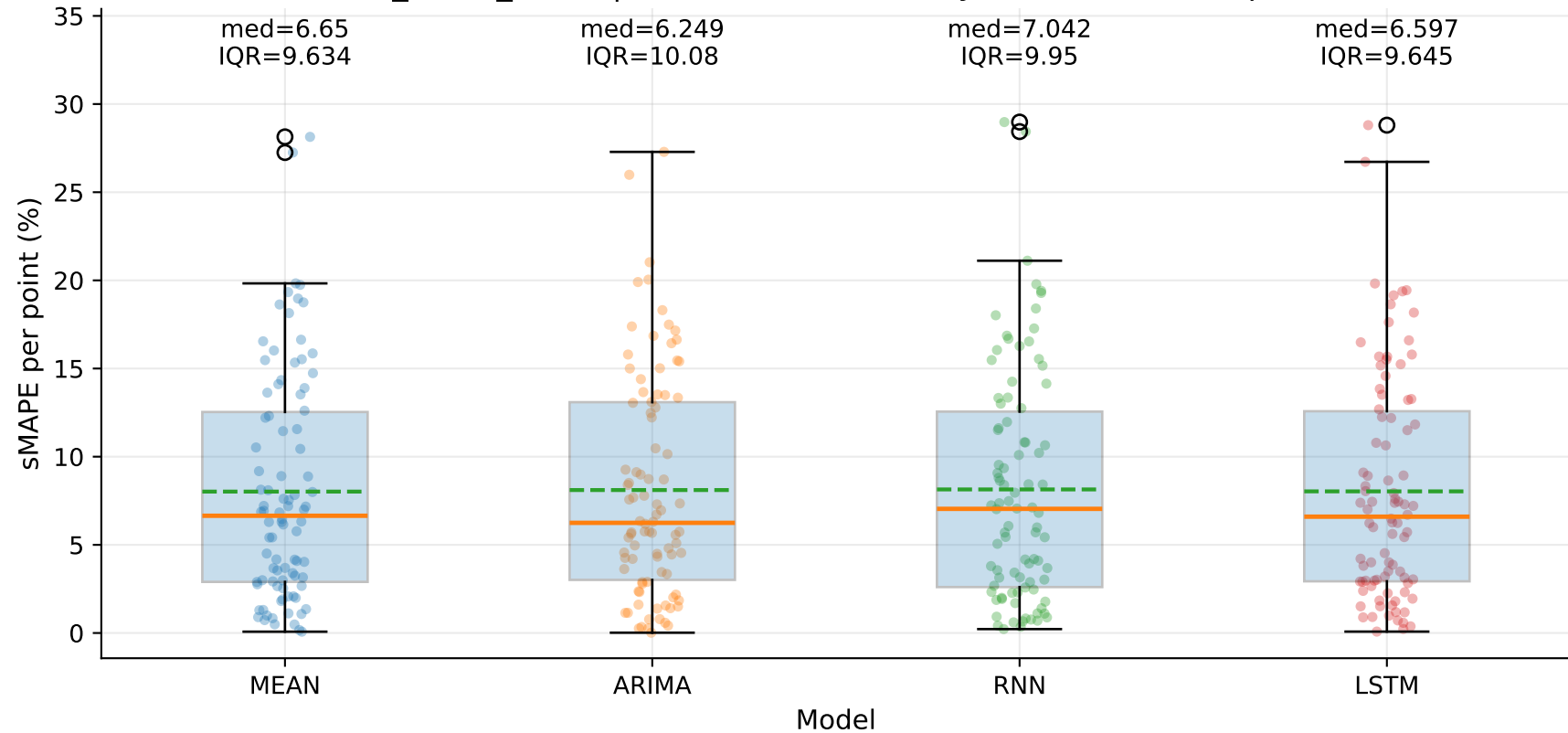
M4_YHUR_SHUR | sMAPE distribution by model — Yd (step=1)
