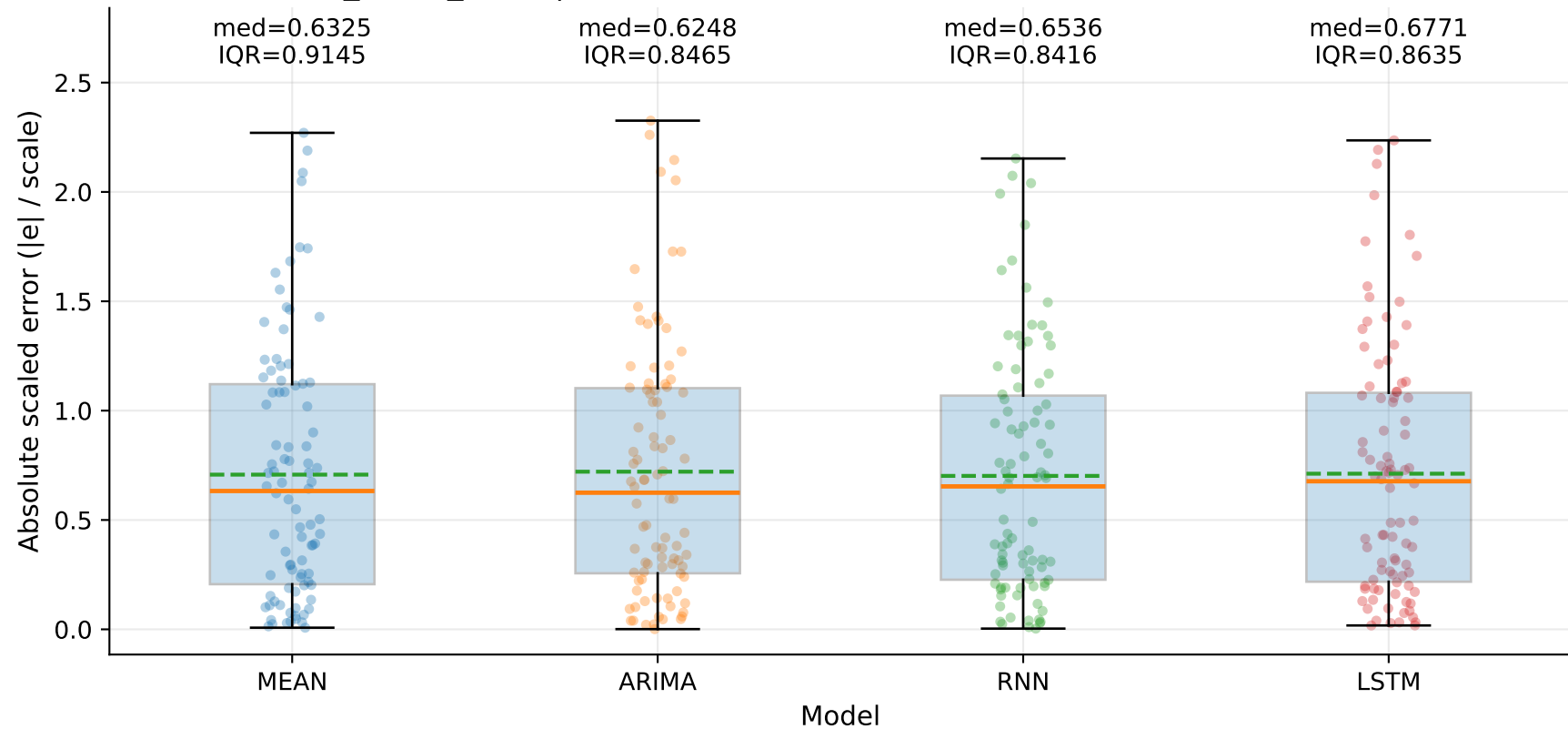
M4_YHUR_SLUR | MASE-point distribution by model — TSEC (step=1)
