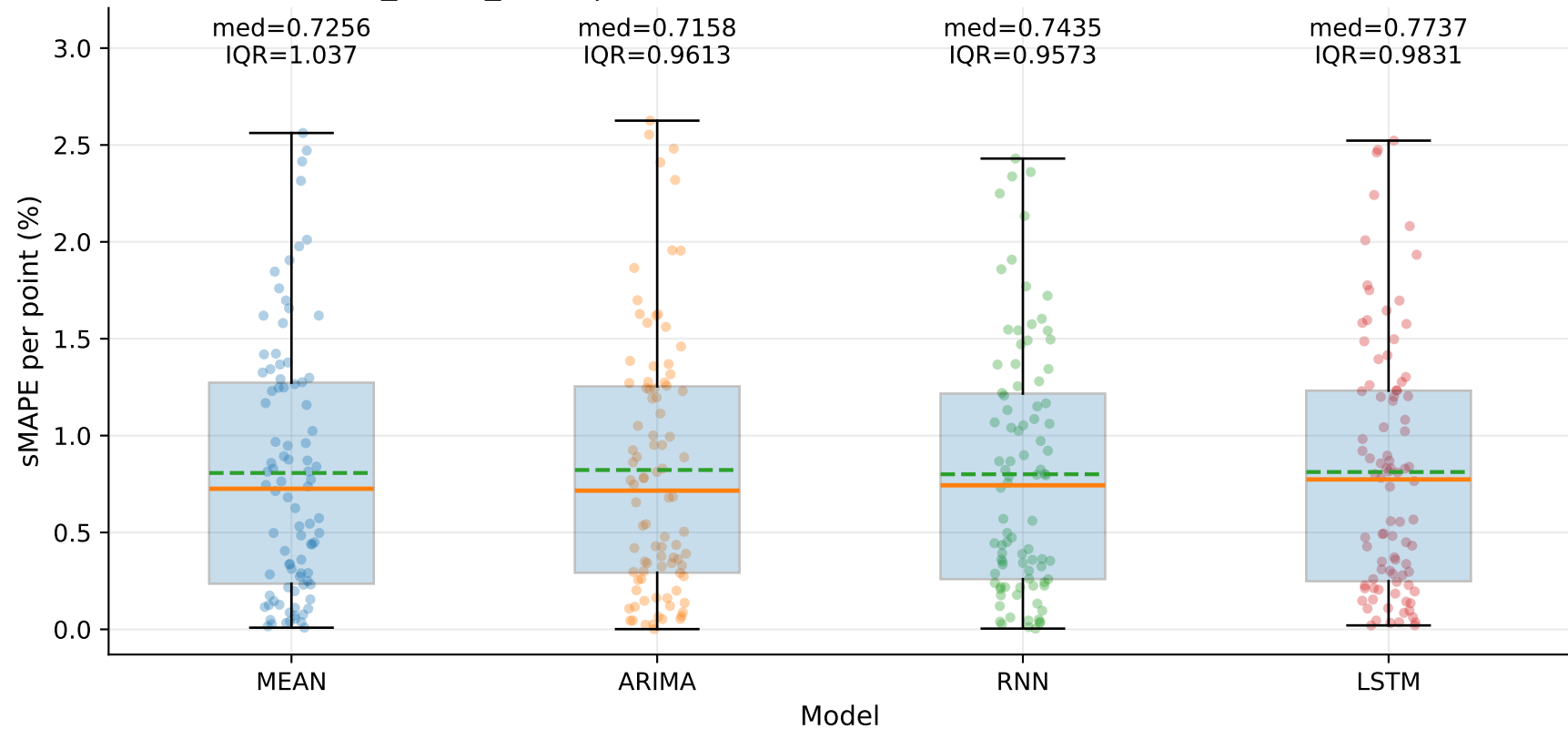
M4_YHUR_SLUR | sMAPE distribution by model — TSEC (step=1)
