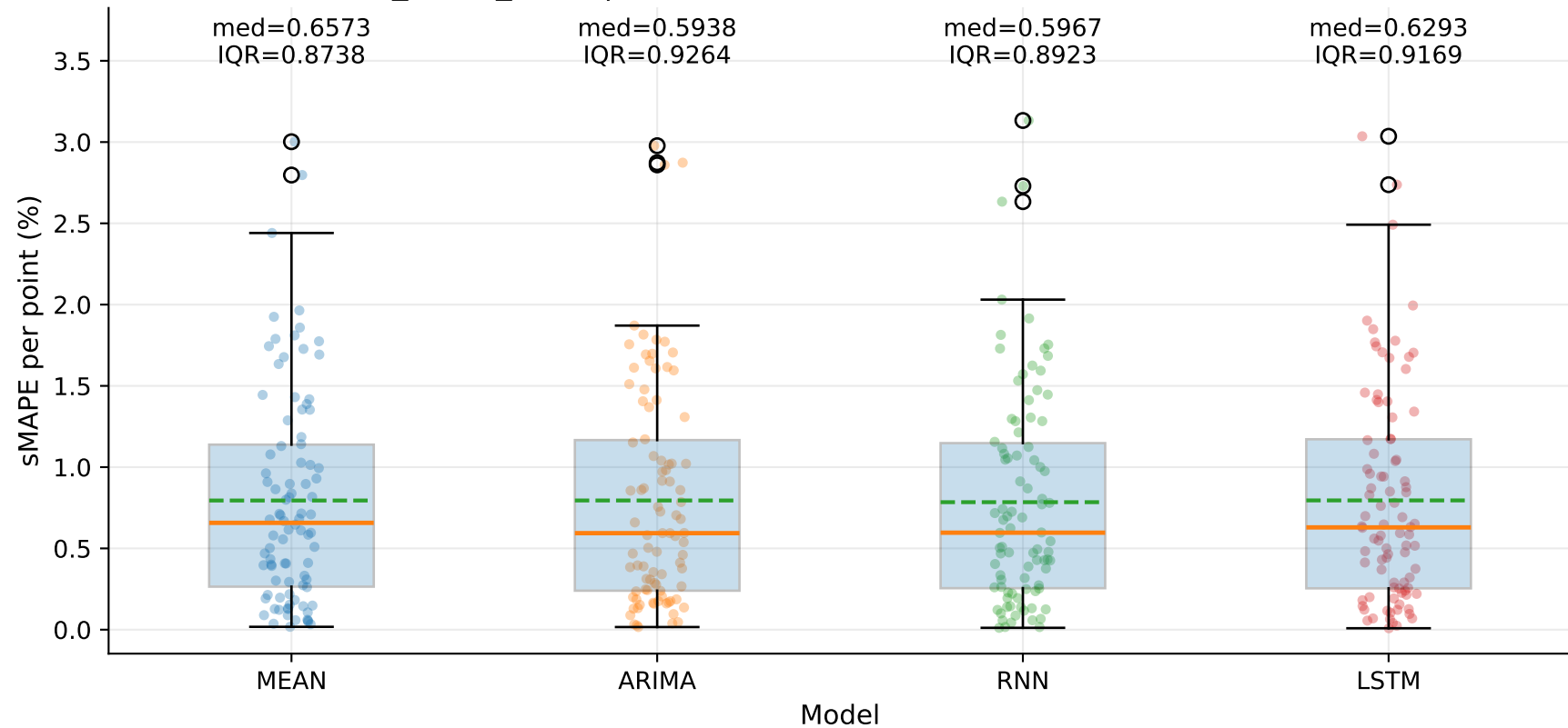
M4_YHUR_SLUR | sMAPE distribution by model — TSE (step=1)
