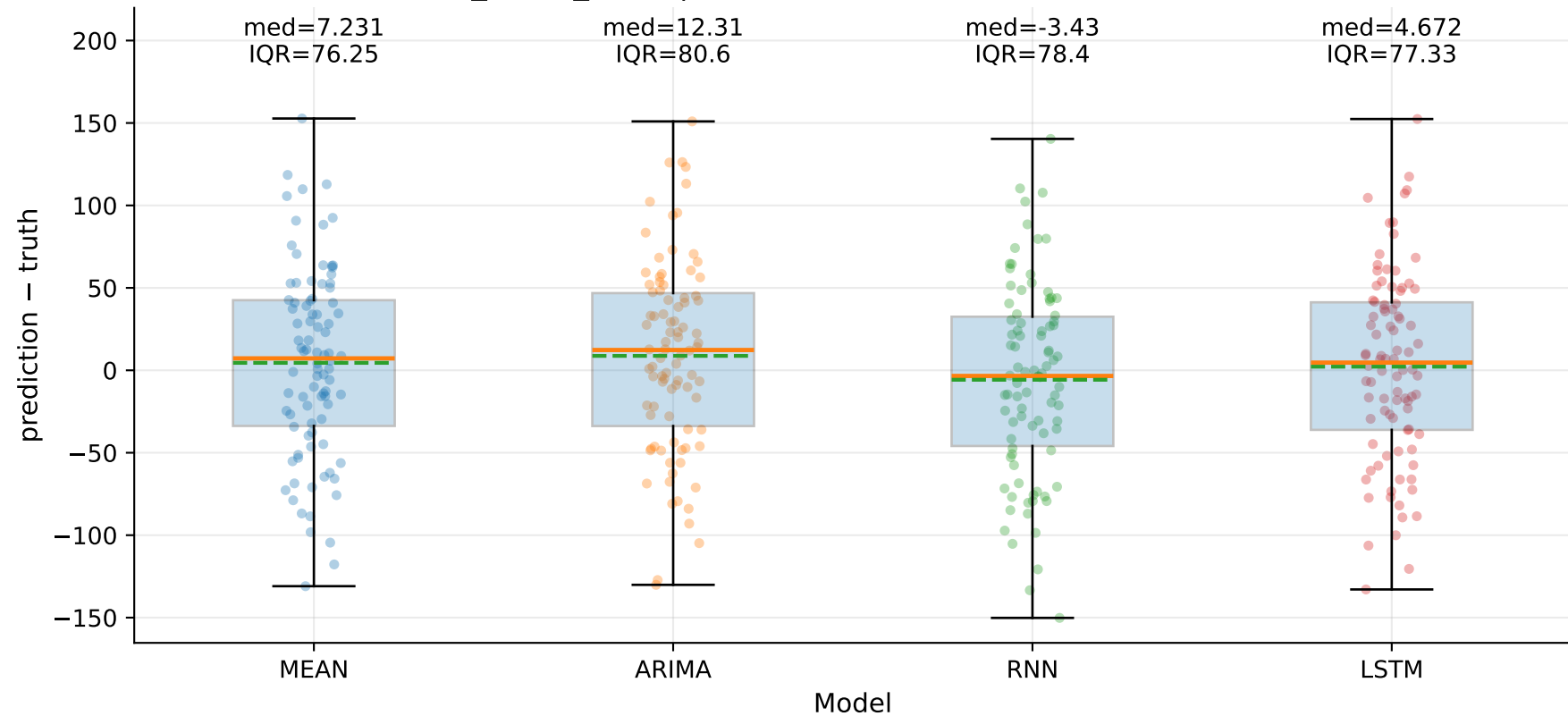
M4_YHUR_SLUR | Signed error by model — Yd (step=1)
