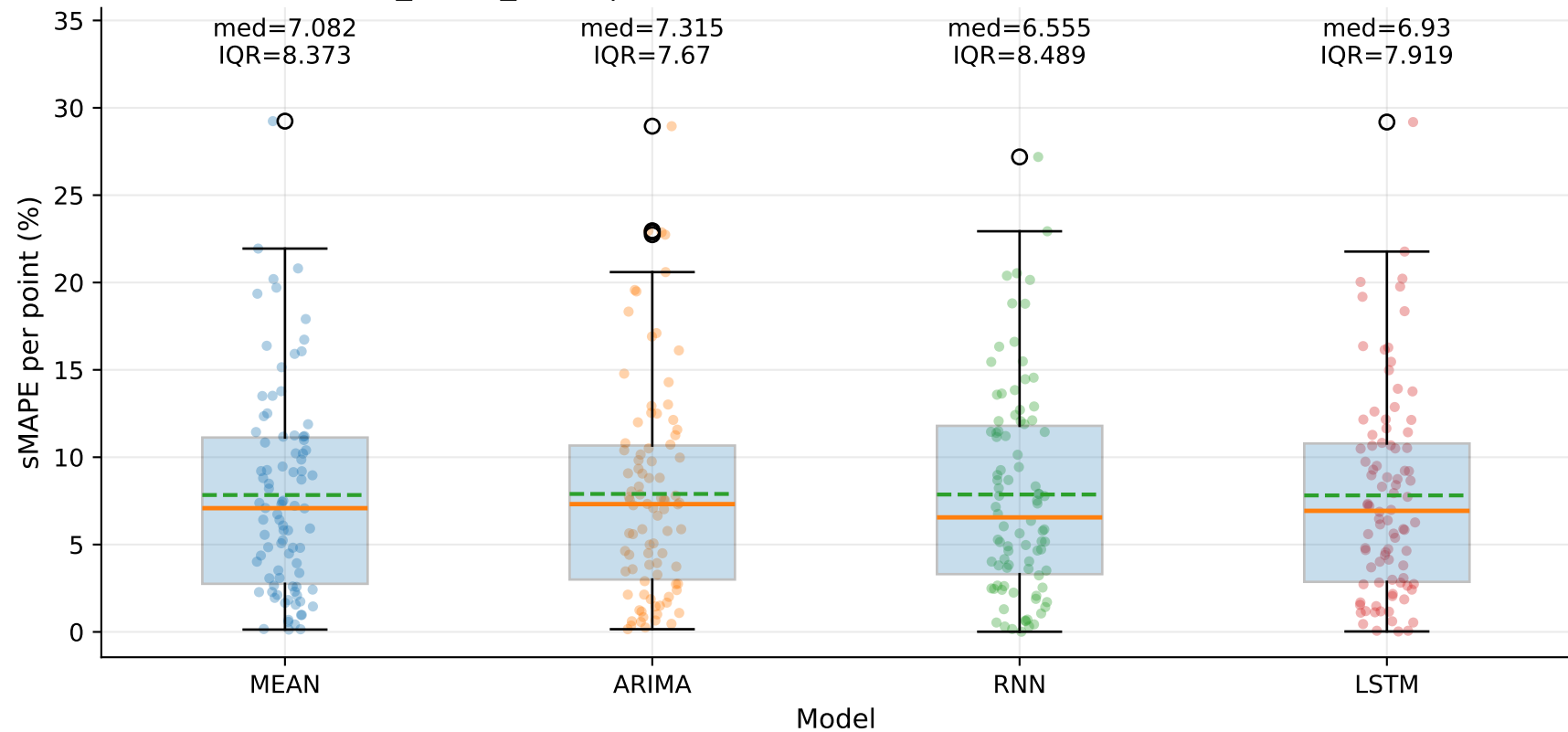
M4_YHUR_SLUR | sMAPE distribution by model — Yd (step=1)
