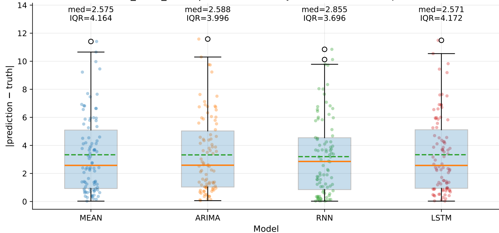
M4_YLUR_SHUR | Absolute error by model — TSEC (step=1)
