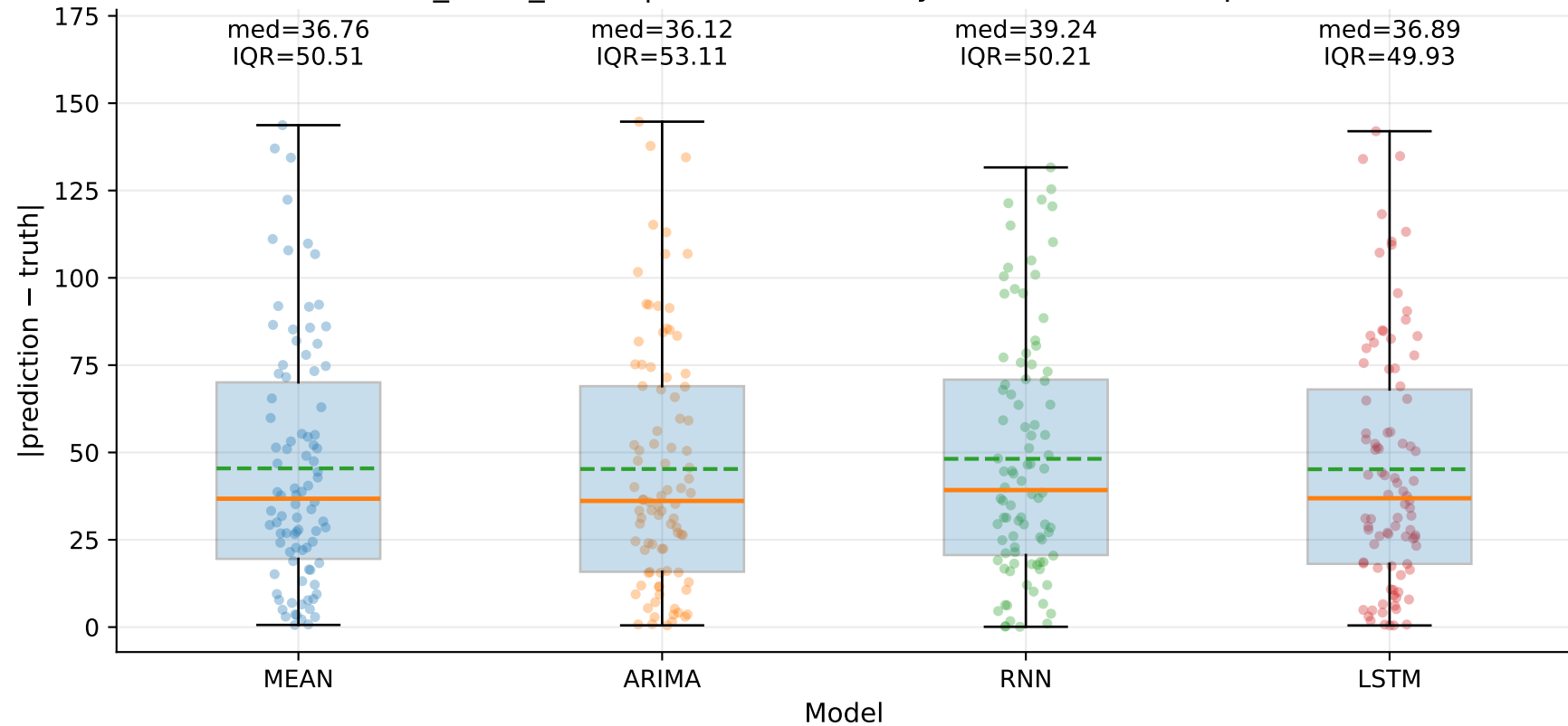
M4_YLUR_SHUR | Absolute error by model — TSE (step=1)
