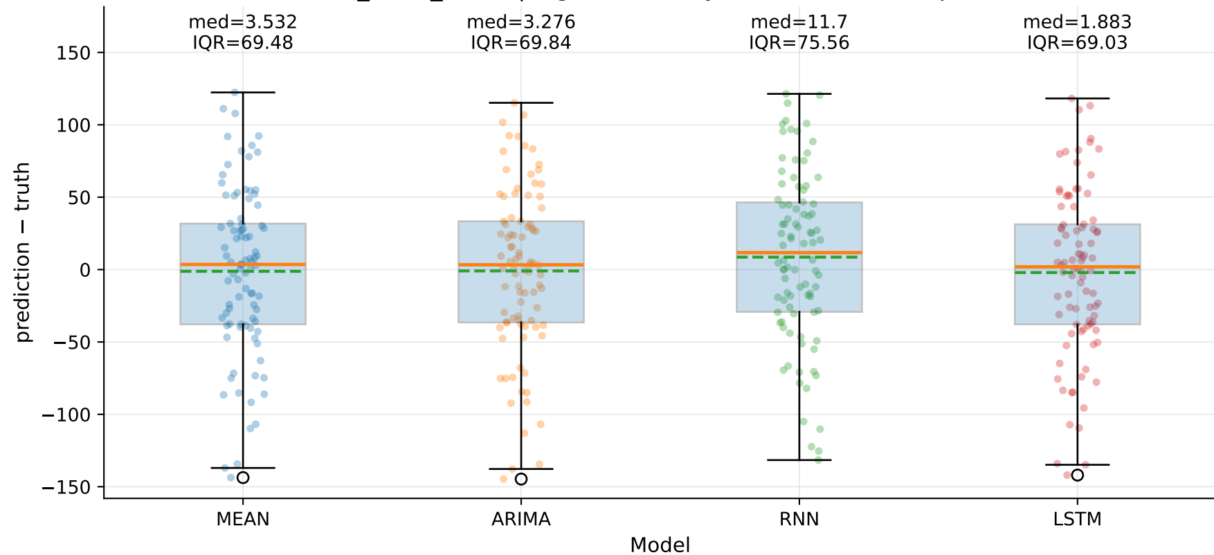
M4_YLUR_SHUR | Signed error by model — TSE (step=1)
