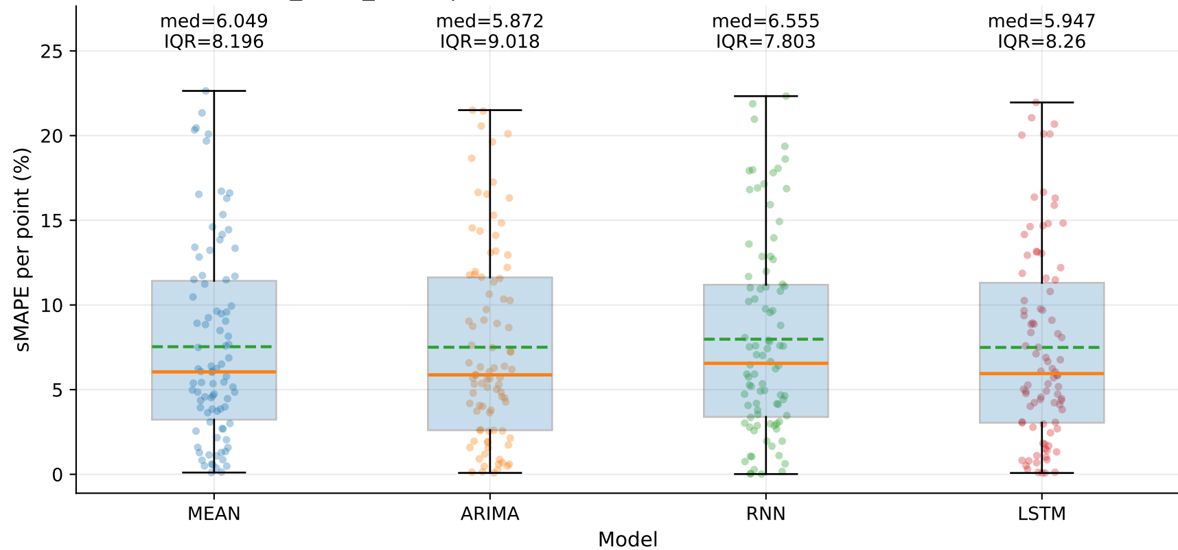
M4_YLUR_SHUR | sMAPE distribution by model — TSE (step=1)
