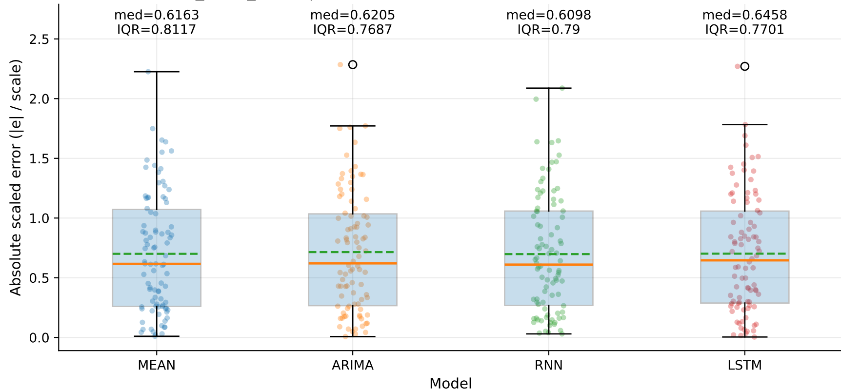
M4_YLUR_SHUR | MASE-point distribution by model — Yd (step=1)
