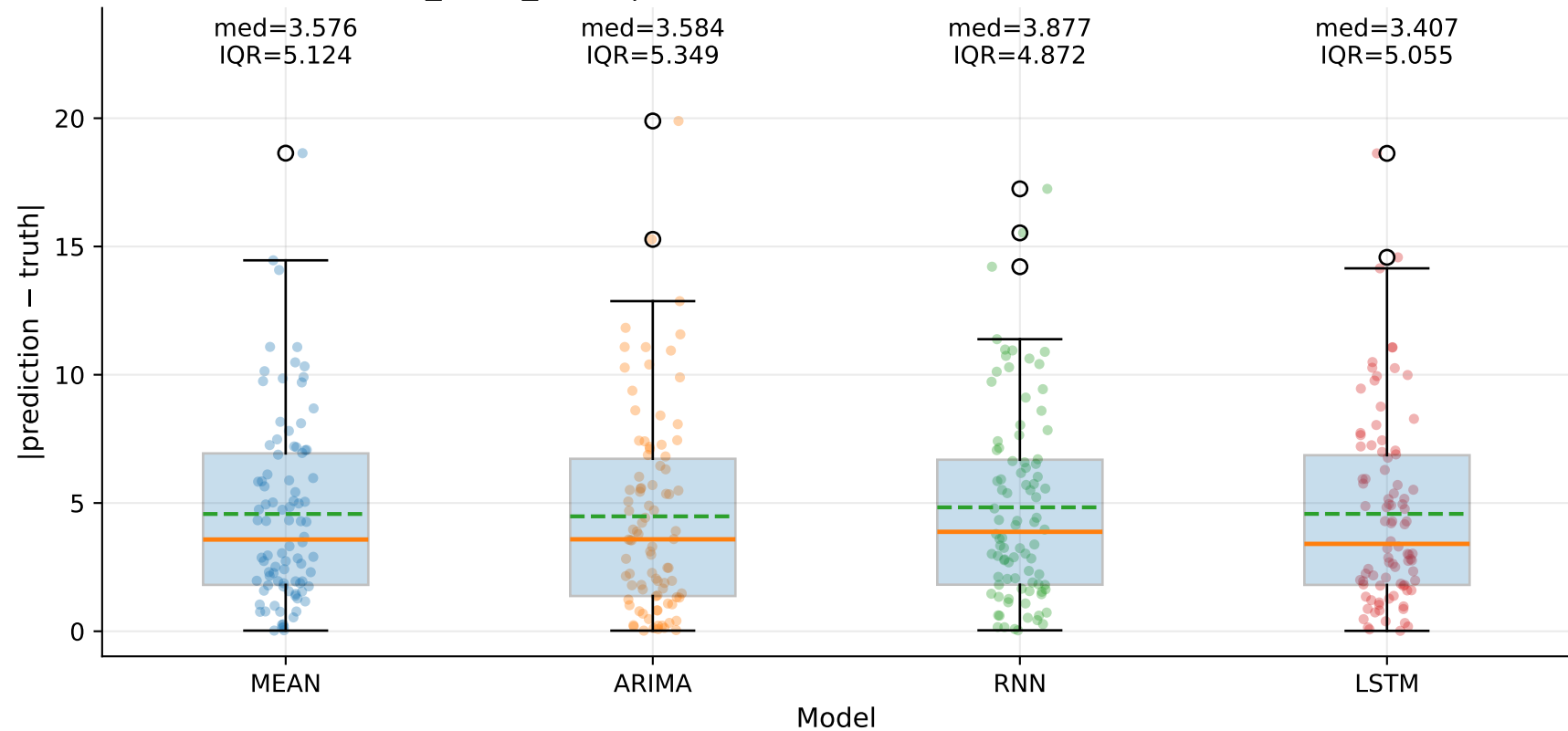
M4_YLUR_SLUR | Absolute error by model — TSE (step=1)
