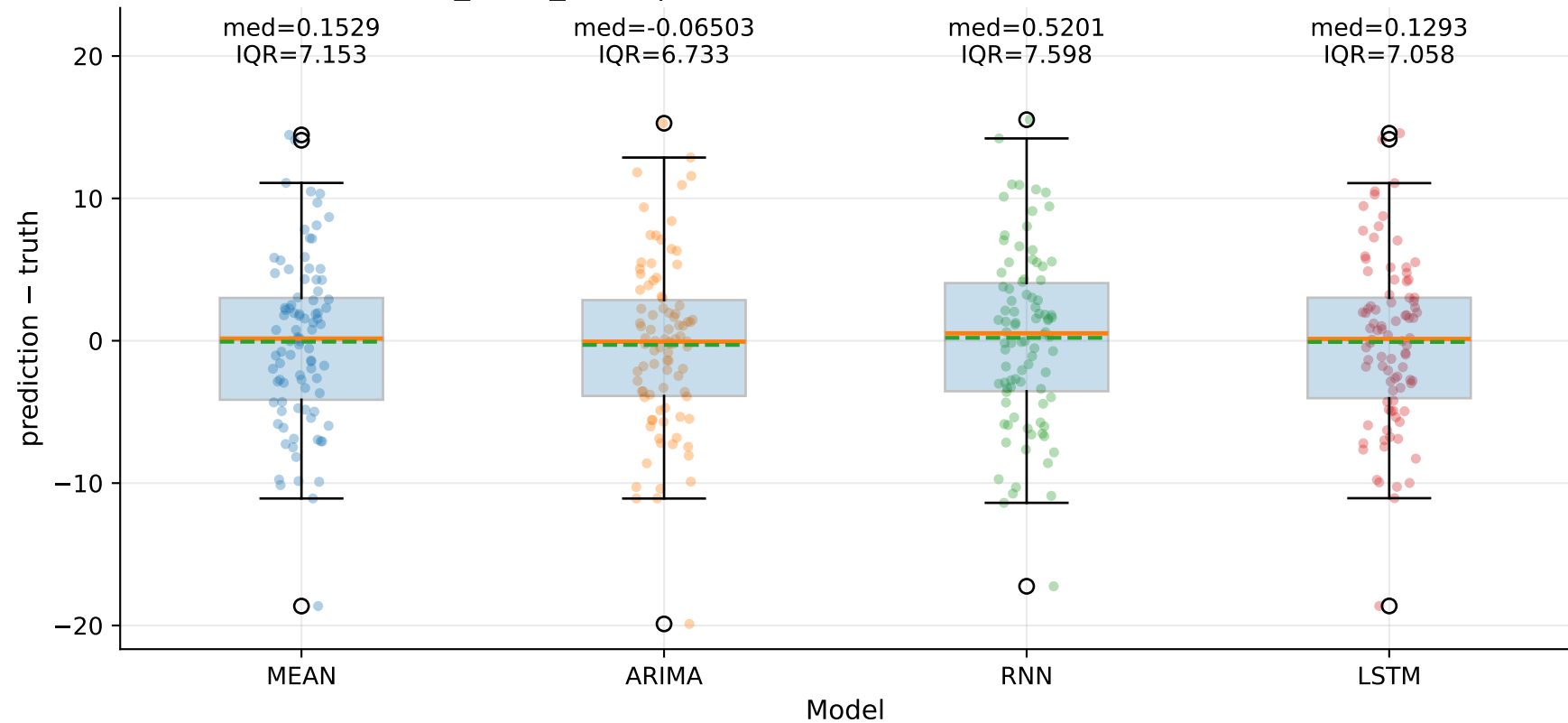
M4_YLUR_SLUR | Signed error by model — TSE (step=1)
