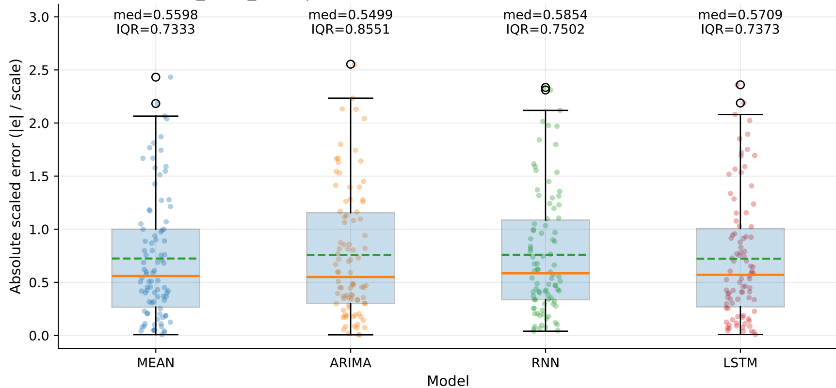
M4_YLUR_SLUR | MASE-point distribution by model — Yd (step=1)
