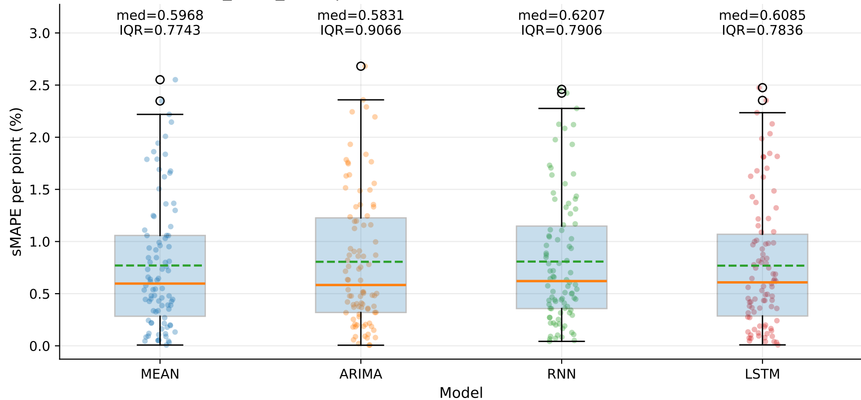
M4_YLUR_SLUR | sMAPE distribution by model — Yd (step=1)
