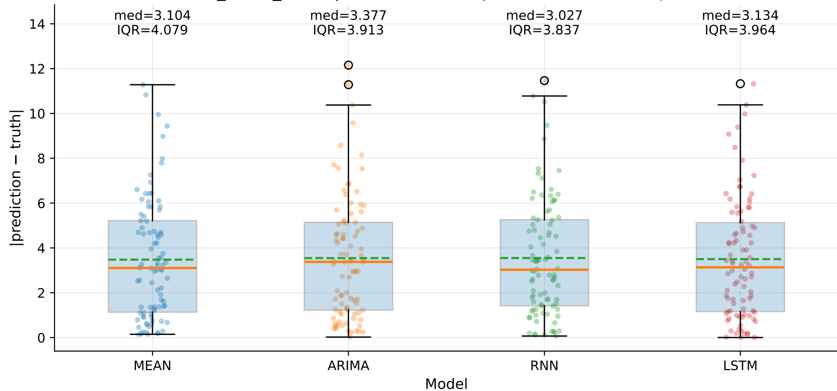
M5_YHUR_SHUR | Absolute error by model — TSEC (step=1)
