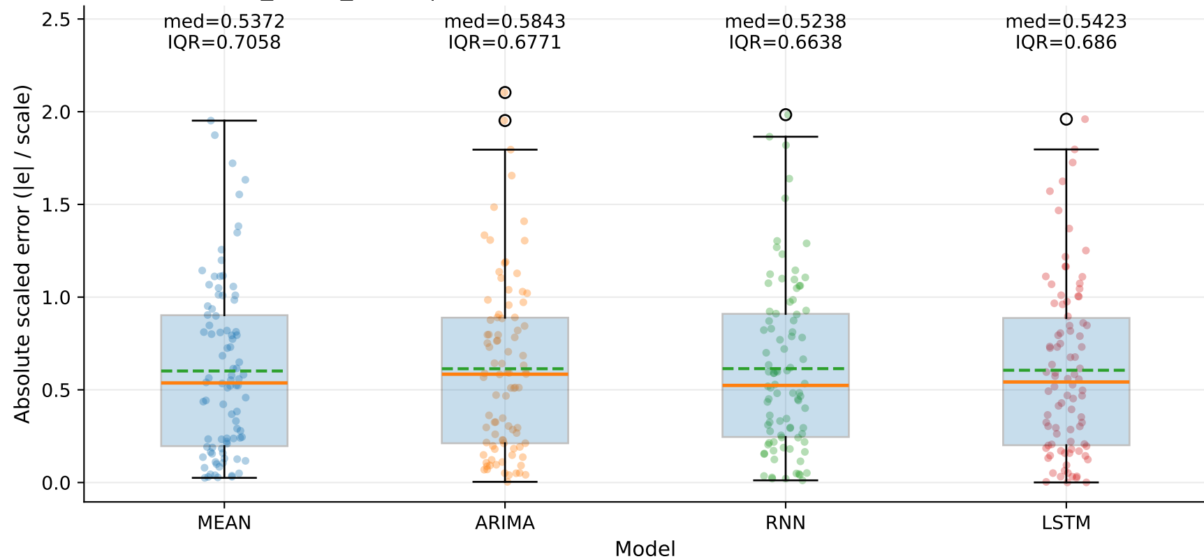
M5_YHUR_SHUR | MASE-point distribution by model — TSEC (step=1)
