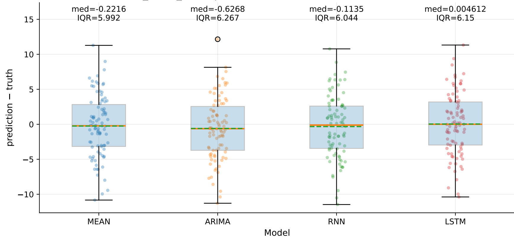
M5_YHUR_SHUR | Signed error by model — TSEC (step=1)
